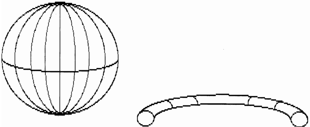
Figure 10-6 Representation of three-dimensional curved surfaces with lines drawn to indicate curvature.
