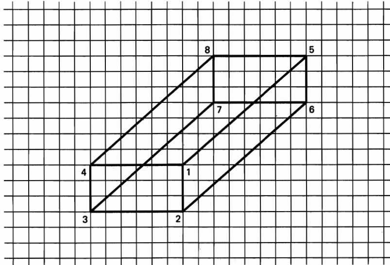
Figure 10-1 Graph paper layout for a three-dimensional box.
