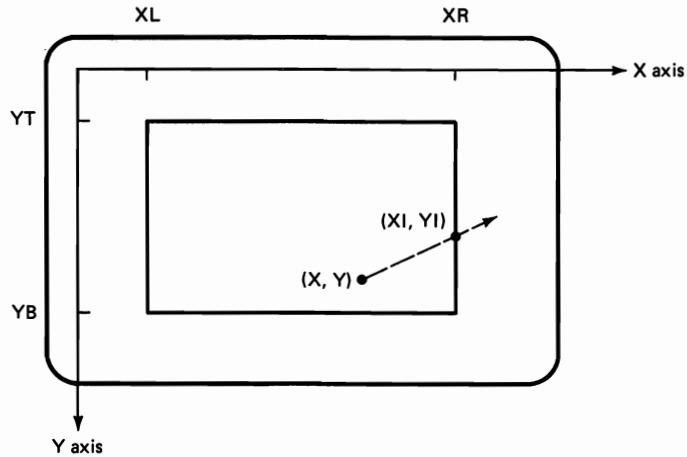
Figure 8-4 A pixel at position (X,Y), traveling along the diagonal path indicated inside a box, will intersect the right boundary at position (XI,YI).
