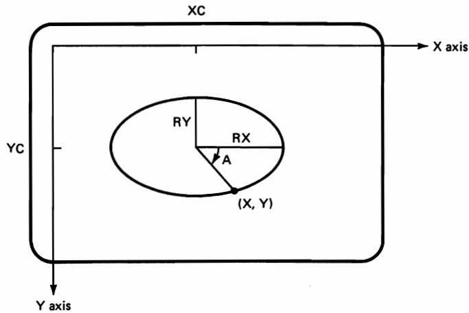
Figure 5-12 An ellipse plotted from equations (5-3) with RX > RY and center at coordinates (XC, YC) .
