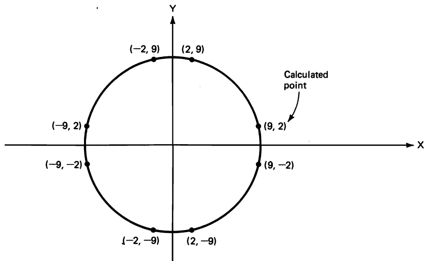
Figure 5-11 If the pixel at location (9,2) is calculated to be on a circle, then all eight points shown can be plotted.
