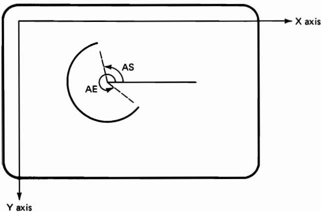
Figure 5-4 A circular arc drawn with the CIRCLE statement from a starting angle AS to an ending angle AE. Angles are measured in a counterclockwise direction from the horizontal.
