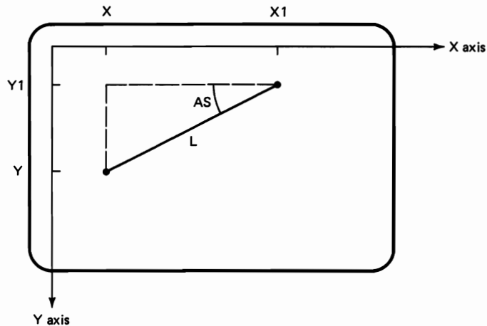
Figure 8-11 Coordinate values (X_1, Y_1) for one end of a line can be calculated from the values for the line length L , the slope angle AS , and the coordinate values (X, Y) of the other end of the line. The slope angle AS is determined from the value for the slope M as AS = \text{ATN}(M) .
