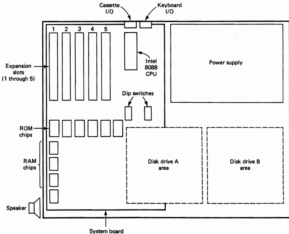
Figure 1-2 System unit layout, showing locations of the system board, power supply, disk drives, and I/O connections.
