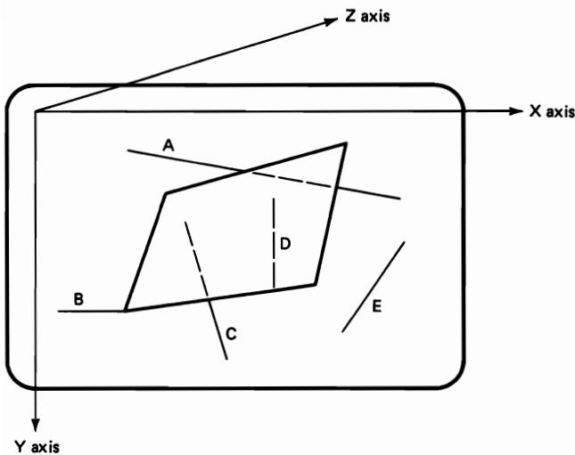
Figure 10-8 Possible line and surface relationships. Line A intersects the face boundary at two points; lines B and C intersect at one point; line D is completely hidden; and line E is completely visible. (All lines are assumed to have greater Z coordinates than the surface.)
