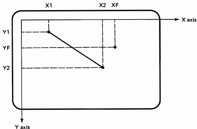
Figure 7-2 A straight line, with horizontal length component X2 - X1 and vertical length component Y2 - Y1 , can be scaled relative to any fixed point (XF,YF).
