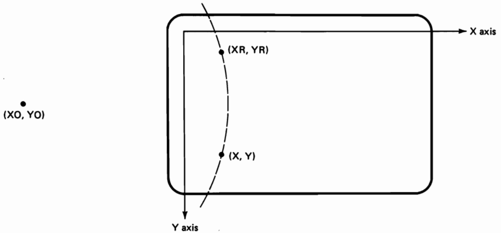
Figure 7-6 Values for the coordinates of the pivot point (XO, YO) can be chosen to be off screen, as well as within the screen coordinate boundaries.
