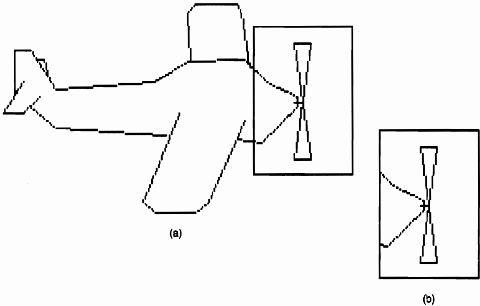
Figure 9-7 Picture displayed (a) before and (b) after clipping by Prog. 9-4.
