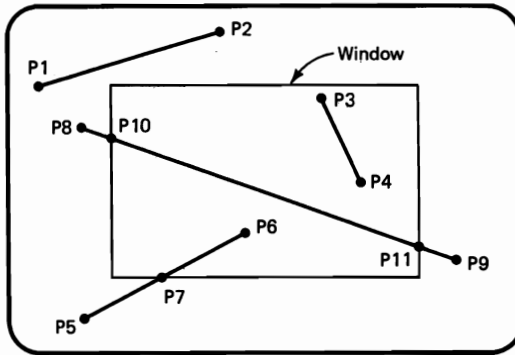
Figure 9-5 A line with endpoint positions P1 and P2, both outside a window, will be erased by the clipping program. A line with endpoints at P3 and P4, both inside the window, will be saved. The clipping routine will also save line segments from P7 to P6 and from P10 to P11.
