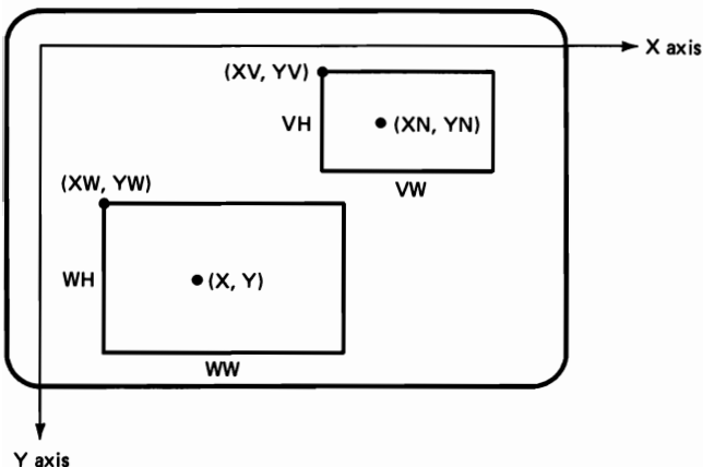
Figure 9-11 Window and viewport specifications. Upper left corner of the window is at position (XW, YW) ; upper left corner of the viewport is at position (XV, YV) . Size of each area is specified by width and height ( WW, WH and VW, VH ). A point with coordinates (X, Y) in the window will be transformed to a new position (XN, YN) in the viewport.
