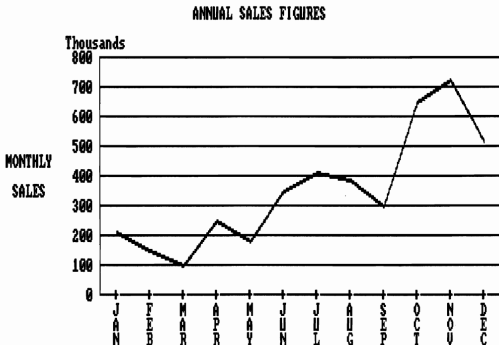
Figure 4-7 Labeled graph with coordinate axes. Output by Prog. 4-6, using pixel graphics methods.
