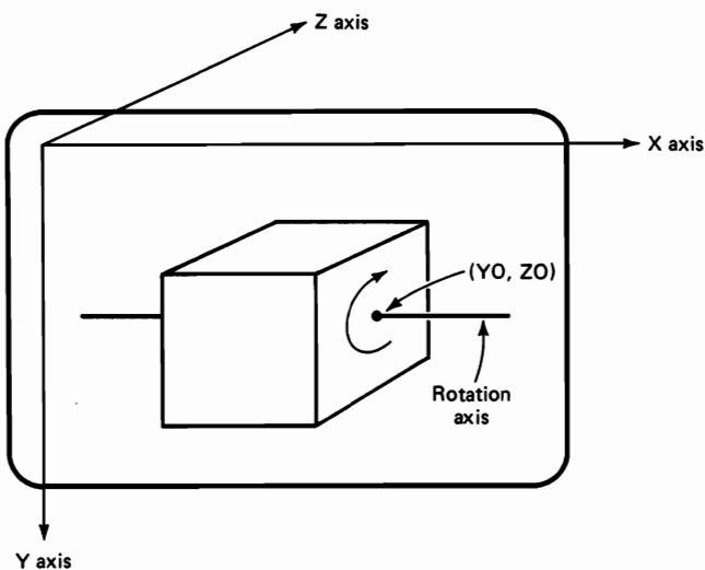
Figure 11-5 Rotating an object about an axis in the X direction changes Y and Z coordinates, while leaving X values unchanged.
