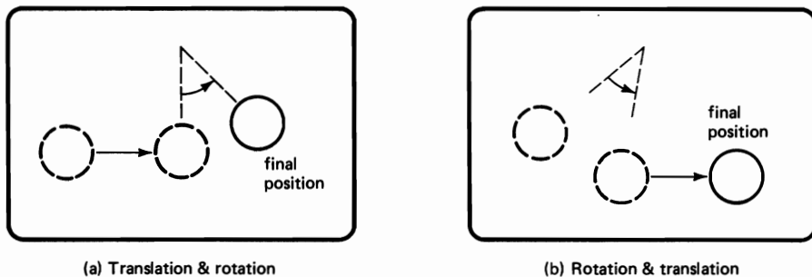
Figure 7-10 Final position of an object after translation and rotation (about a point external to the object) depends on the order of these transformations. In (a), translation is performed first; in (b), translation is performed last.
