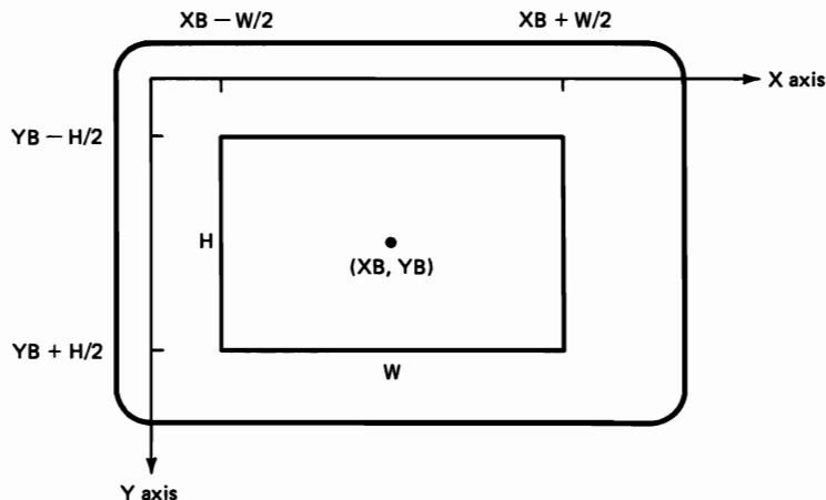
Figure 9-2 Coordinates for the corners of a rectangle can be determined from values for the width W , height H , and center position (X_B, Y_B) .
