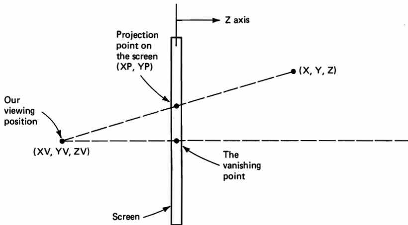
Figure 10-12 A point with coordinates (X, Y, Z) is projected onto the screen at position (XP, YP) by a perspective transformation when our viewing position is at (XV, YV, ZV) .
