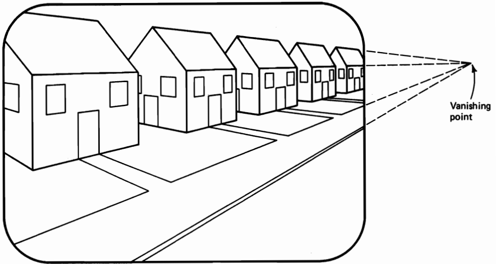
Figure 10-11 In a perspective view, parallel lines are redrawn to converge to a vanishing point so that distant objects are displayed smaller than nearer objects.
