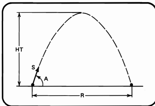
Figure 8-9 An object tossed into the air with initial speed S at an angle A will rise to height HT and land a distance R away from the starting point. Both the range R and height HT are calculated from values for the projection speed S and projection angle A .
