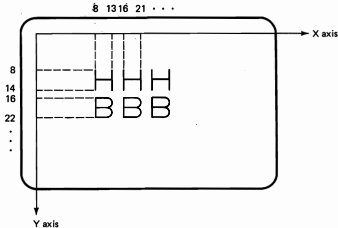
Figure 9-9 Coordinate positions for characters with an 8 by 8 pixel grid. Horizontally, characters start at pixel locations 0, 8, 16, ... and end at pixel locations 5, 13, 21, and so on across the screen. Tops of the print lines are at pixel positions 0, 8, 16, ... , and bottoms of the print lines are at pixel positions 6, 14, 22, and so on down the screen.
