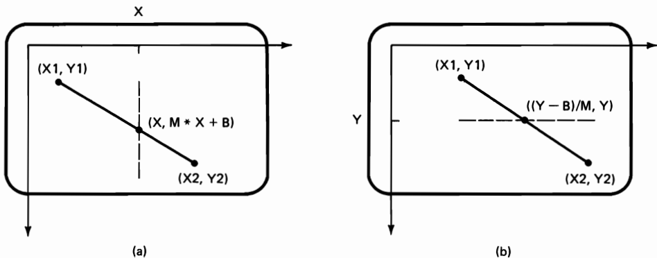
Figure 9-6 Line with slope M and Y -intercept B crossing vertical and horizontal boundaries: (a) intersection with the vertical boundary is at coordinates (X, M * X + B) ; (b) intersection with the horizontal boundary is at coordinates ((Y - B)/M, Y) .
