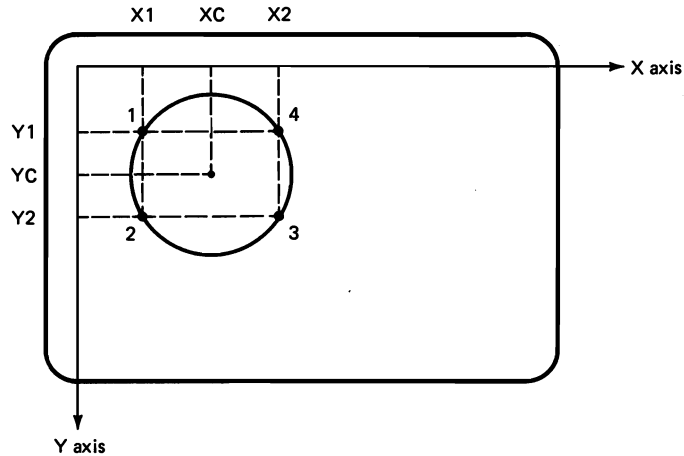
Figure 5-10 Symmetry of a circle. Points 1 and 2 have the same X value; points 1 and 4 have the same Y value.
