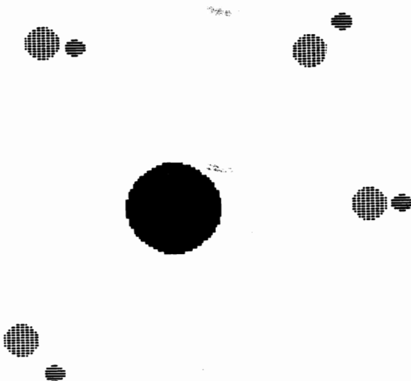
Figure 13-3 Simulation of the motion of the earth and moon about the sun, showing several positions from the output of Prog. 13-2.
