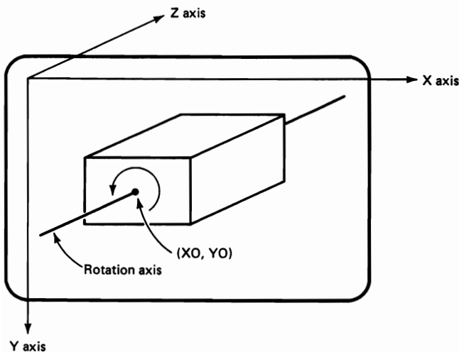
Figure 11-3 Rotating an object about an axis in the Z direction changes X and Y coordinates, but leaves Z coordinates unchanged.
