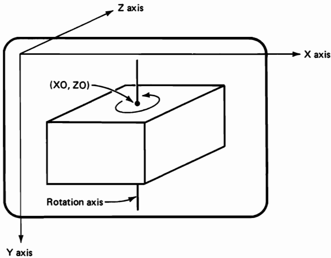
Figure 11-4 Rotating an object about an axis in the Y direction changes X and Z coordinates, but leaves Y coordinates unchanged.
