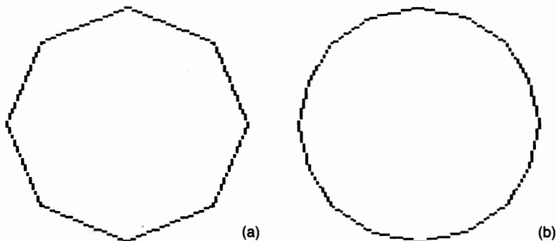
Figure 5-7 Circle approximated with (a) 8 straight line segments and (b) 16 line segments, by Prog. 5-2.
