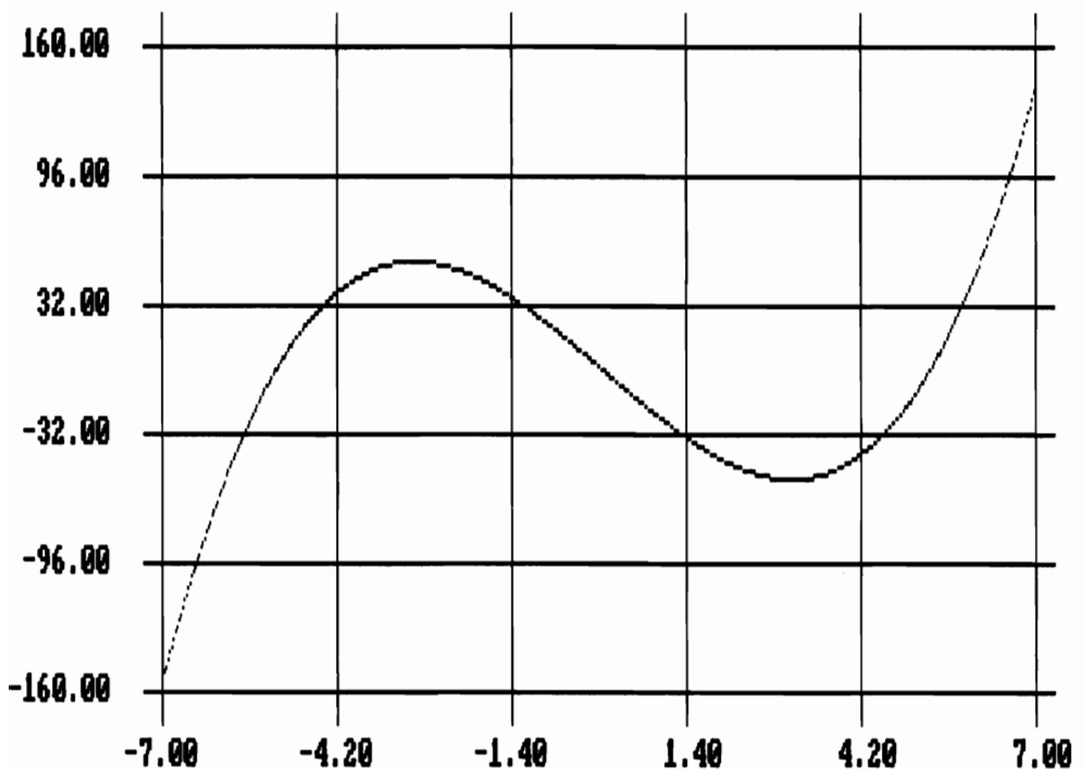
Figure 5-20 Graph of the function X^3 - 27 * X , output by Prog. 5-10.
