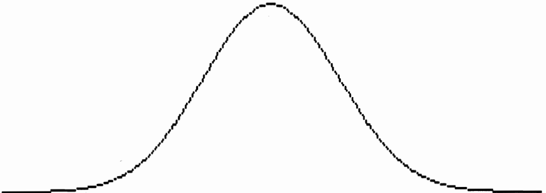
Figure 5-16 Normal probability curve plotted with M = 51.8 and S = 29.2 by Prog. 5-6.
