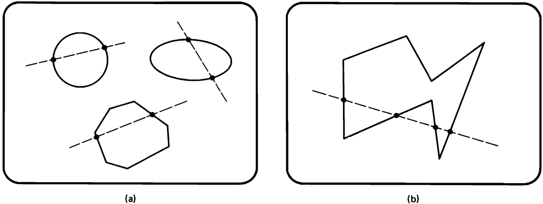
Figure 10-9 (a) Circles, ellipses, and convex polygons (interior angles less than 180 degrees) have no more than two intersection points with a straight line. (b) Concave polygons (interior angles greater than 180 degrees) can have more than two intersection points with a straight line.
