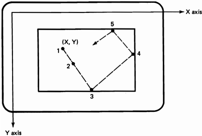
Figure 8-3 Path of a bouncing pixel inside a box. Starting from coordinates (X, Y) at position 1, the pixel will have coordinates (X+DX, Y+DY) at position 2. At position 3, the direction of travel changes by setting DY = -DY . The direction of motion is changed again at position 4 with DX = -DX , and at position 5 with DY = -DY .
