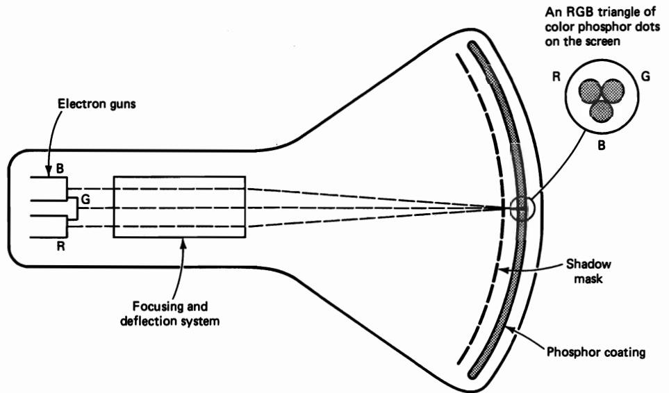
Figure 1-5 Shadow-mask CRT. Three electron guns, arranged in a pattern to coincide with the arrangement of each triangle of color dots on the screen, are directed onto the dot triangles by a shadow mask. The mask allows only the electrons from the B gun to strike the B dot, the R gun to strike the R dot, and the G gun to strike the G dot.
